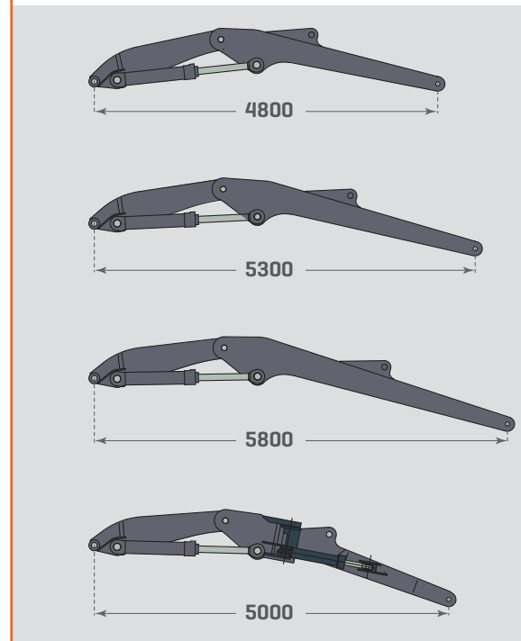
ADJUSTMENT EQUIPMENT
