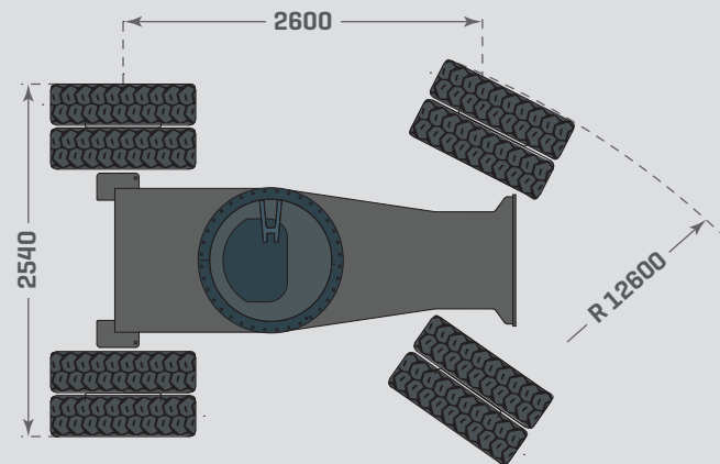
AXLE ZF 3060. TIRE 10.00-20
